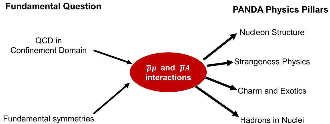
Fig. 1 The PANDA physics domains emerging when using antiproton interactions with nucleons and nuclei as diagnostic tools to shed light on some of the most challenging unresolved problems of contemporary physics
